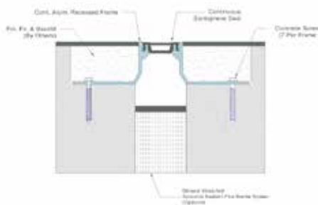
Series i330-25 - Mineral Wool & Sealant Fire Barrier Options
