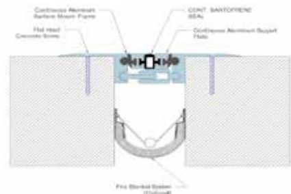
Series i325-50 - Fire Blanket System
