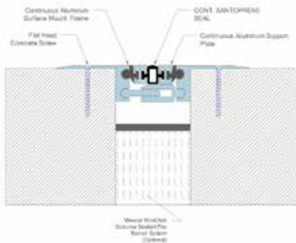
Series i325-50 - Mineral Wool & Sealant Fire Barrier Options
