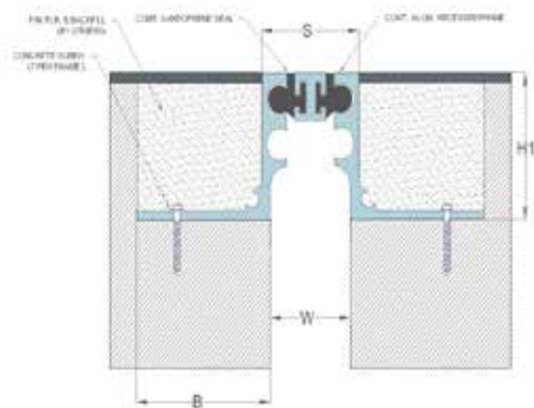
Series i320-25 - Mineral Wool & Sealant Fire Barrier Options
