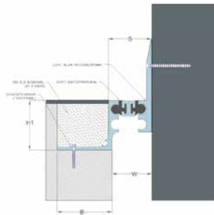
Series i320-C-25 - Floor to Wall
